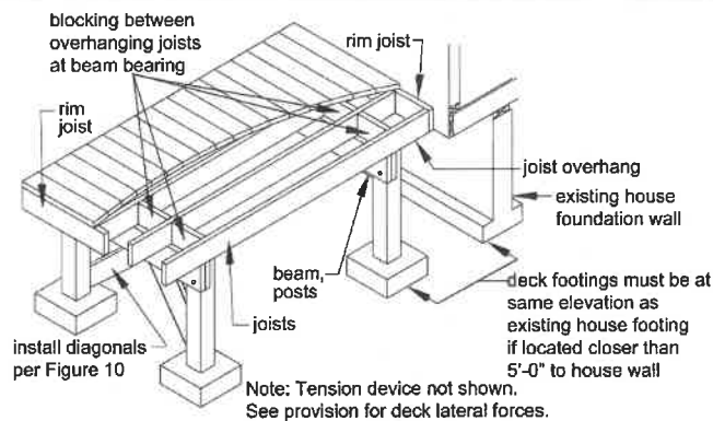
Figure 21. Non-Ledger Deck - For Resisting Vertical Loads.
