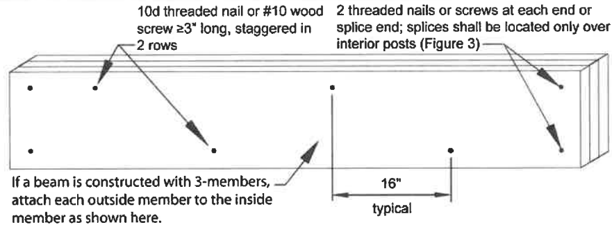
Figure 4. Beam Assembly Details.
