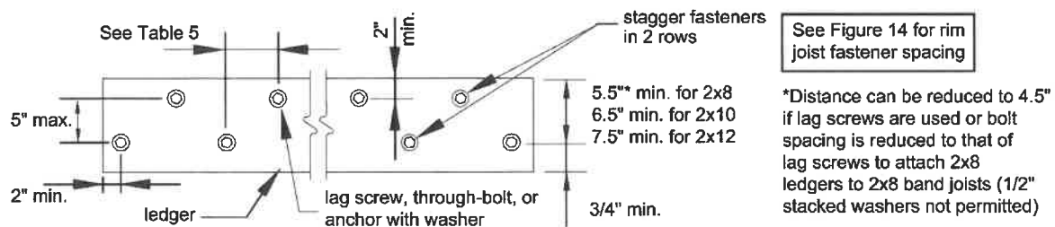
Figure 19. Ledger Board Fastener Spacing and Clearances.
