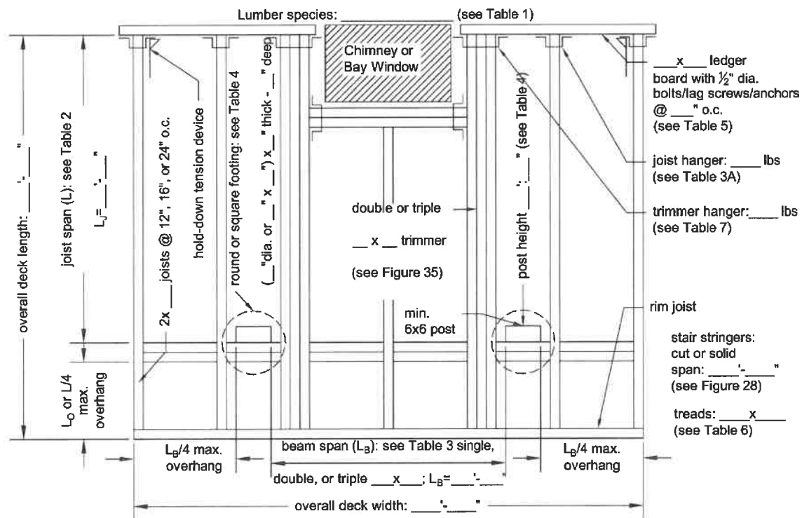
Figure 5. Typical Deck Framing Plan.
