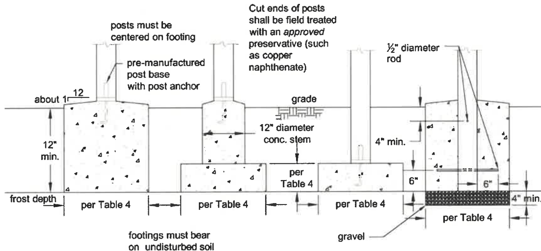
Figure 12. Typical Footing Options.
