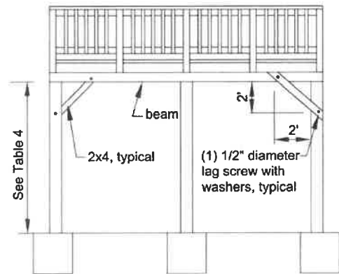
Figure 10. Diagonal Bracing.
