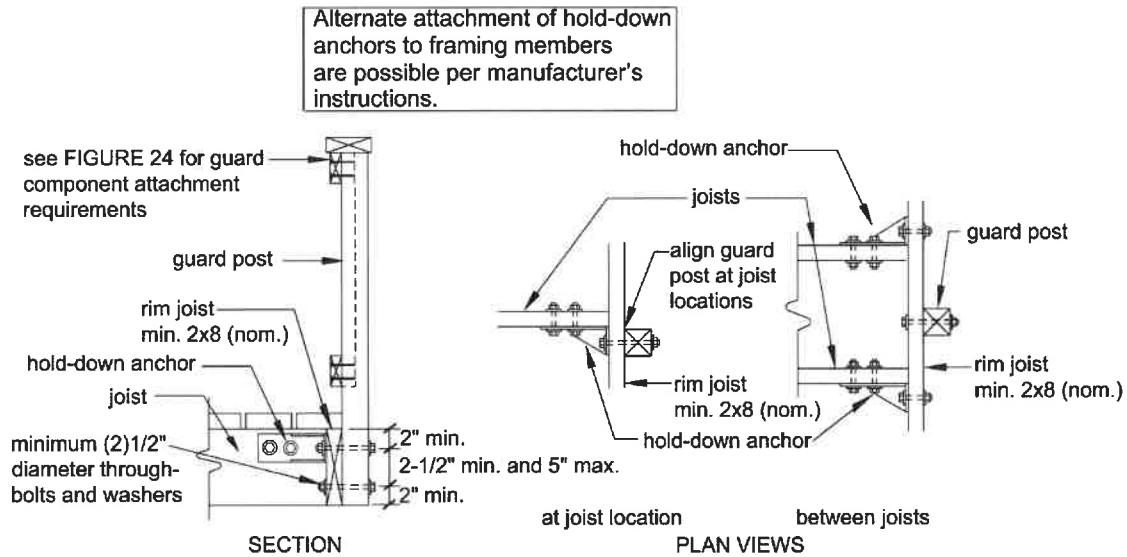
Figure 26. Guard Post to Rim Joist Example.
