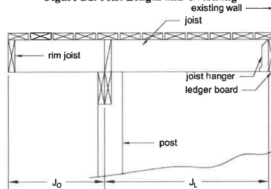
Figure B2. Joist Length and Overhang
