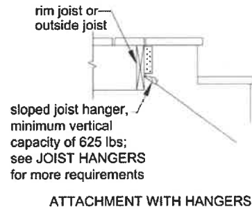
Figure 31. Stair Stringer Attachment Detail.
