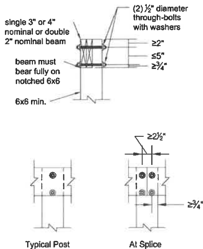
Figure 8A. Post-to-Beam Attachment Requirements.
