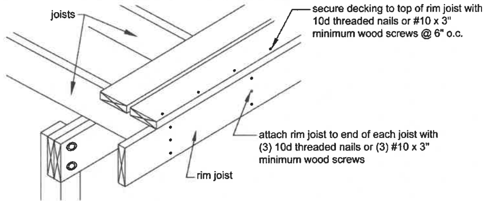
Figure 11. Rim Joist Connection Details.
