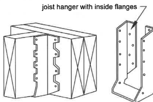
Figure 7. Typical Joist Hangers.
