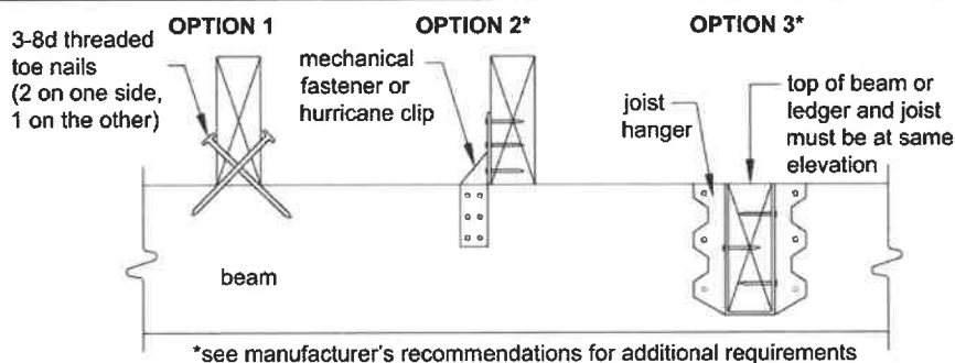
Figure 6. Joist-to-Beam Detail.
