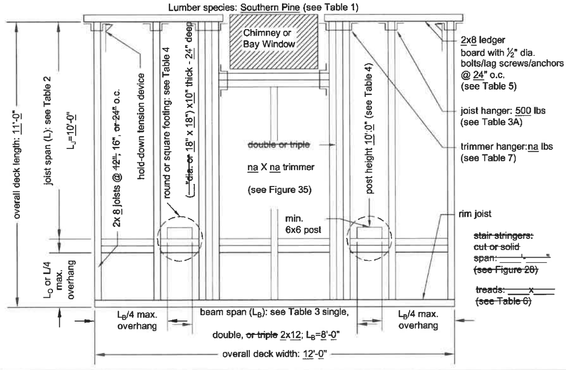
Figure C5. Example of a Typical Deck Framing Plan.
