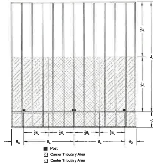
Figure B1. Examples of Tributary Areas
