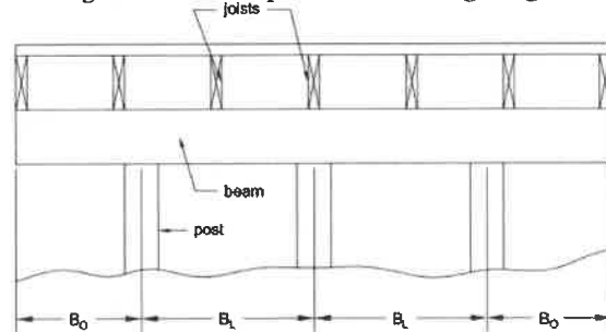
Figure B3. Beam Span and Overhang Length
