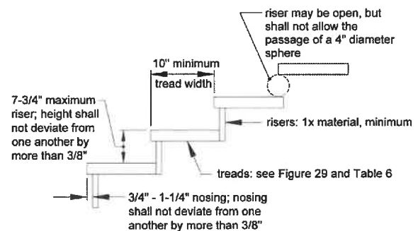
Figure 27. Tread and Riser Detail.
