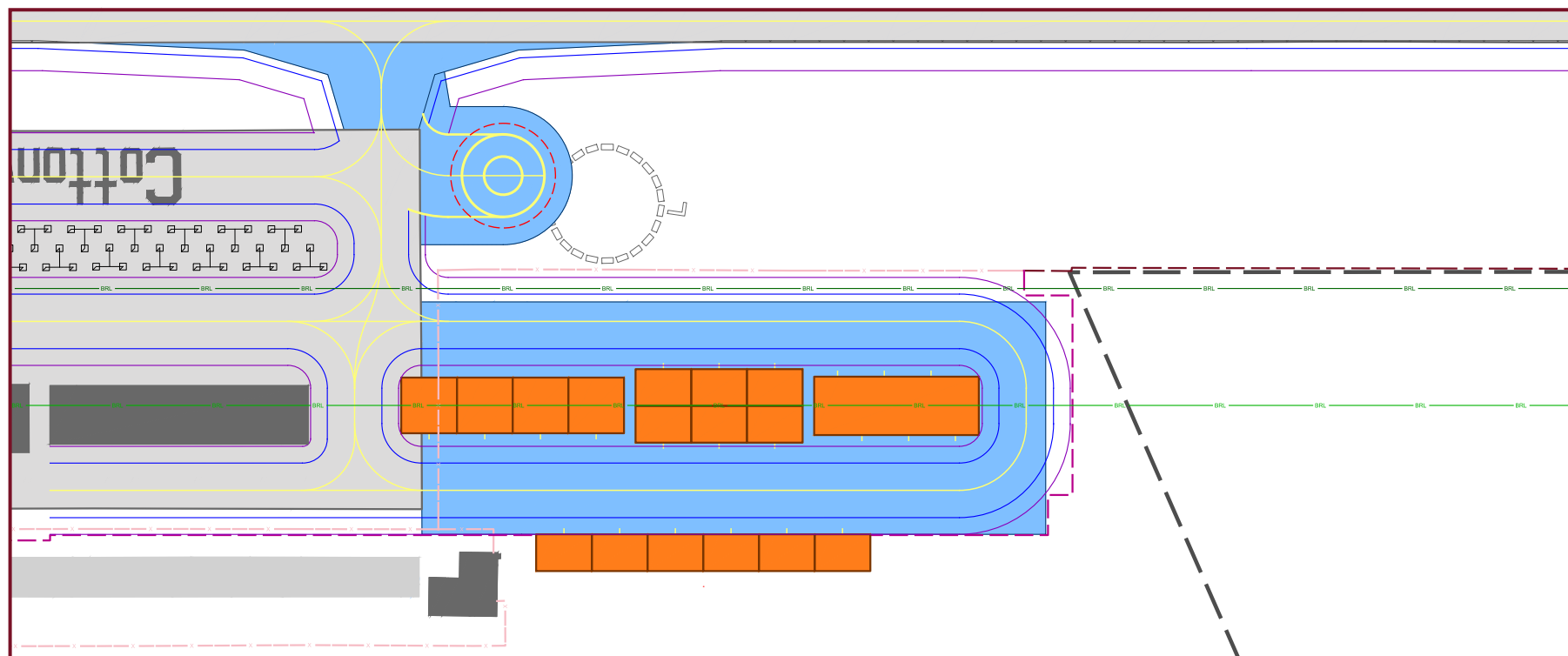
Figure 4.16 - Hangar Development Alternative 2
