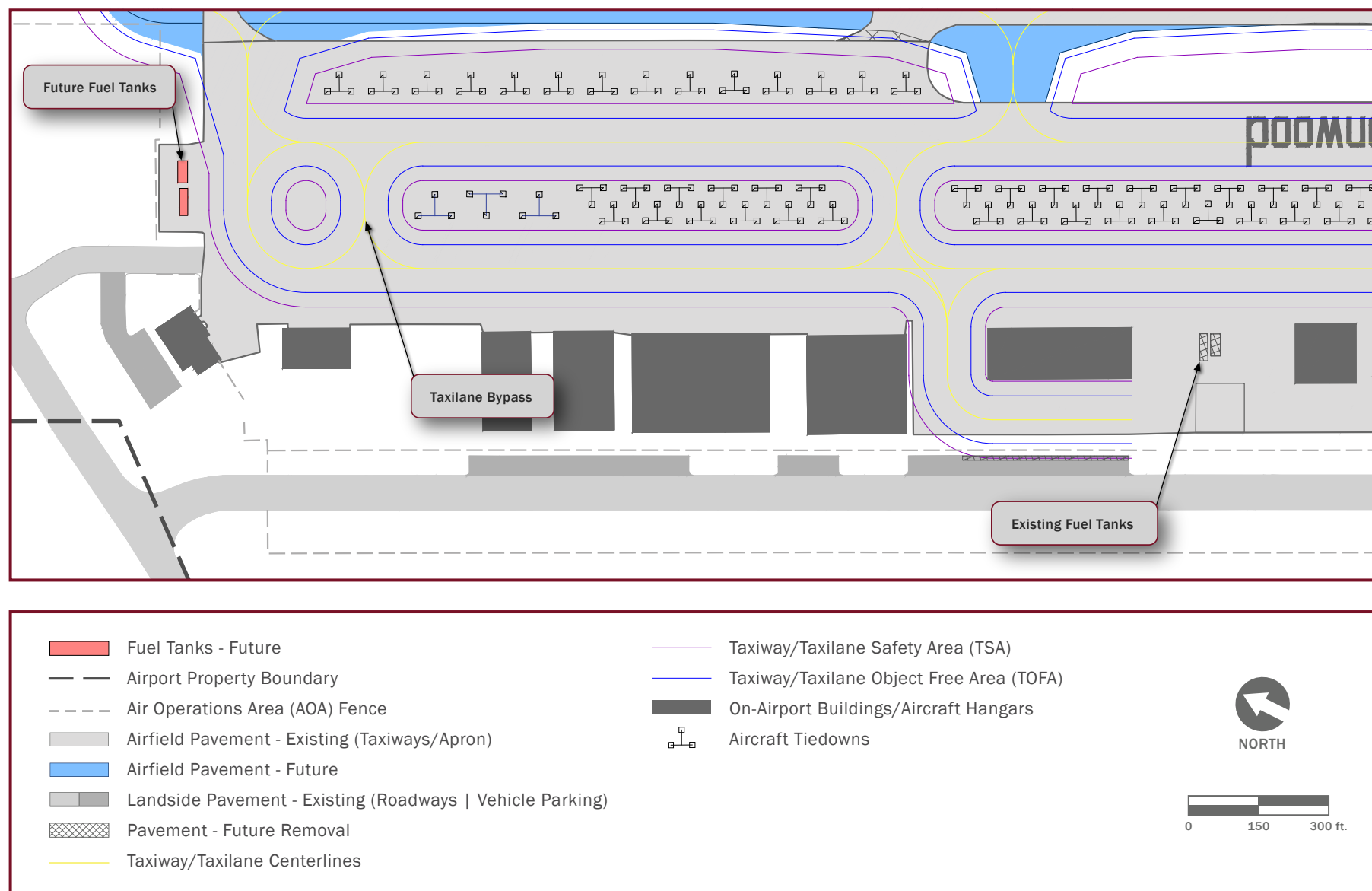
Figure 4.9 - Fuel Tank Alternative 1b
