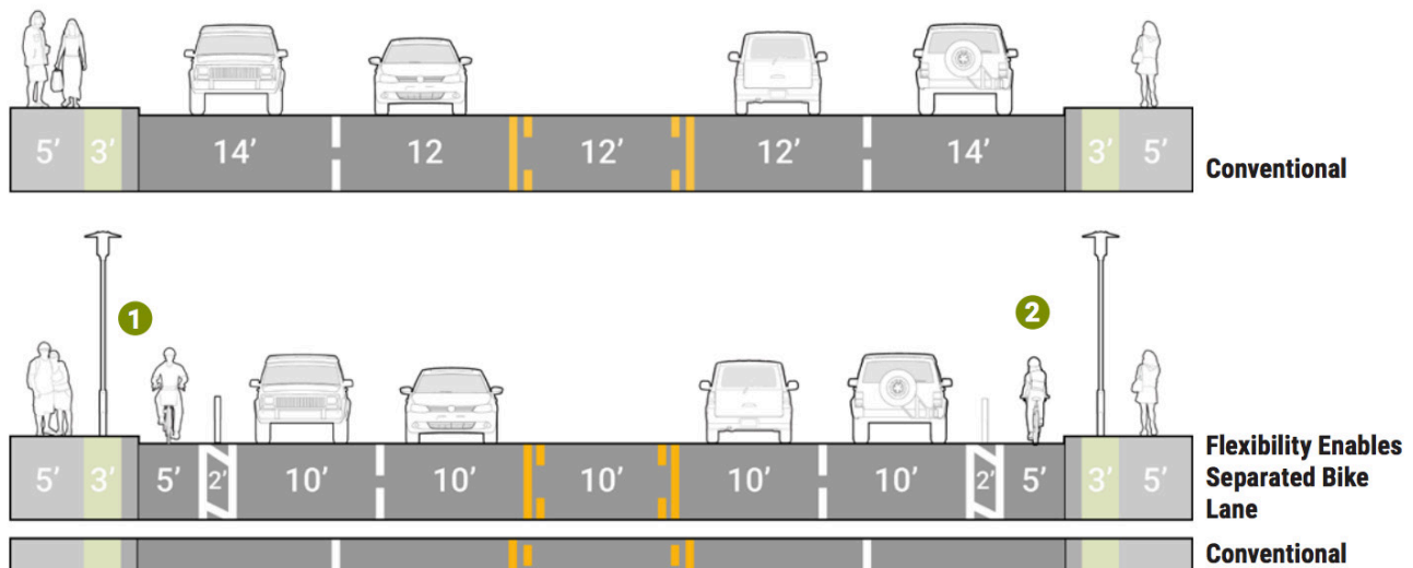
FIGURE 13. SEPARATED BIKE LANES, 5-LANE ROADWAY RECONFIGURATION
