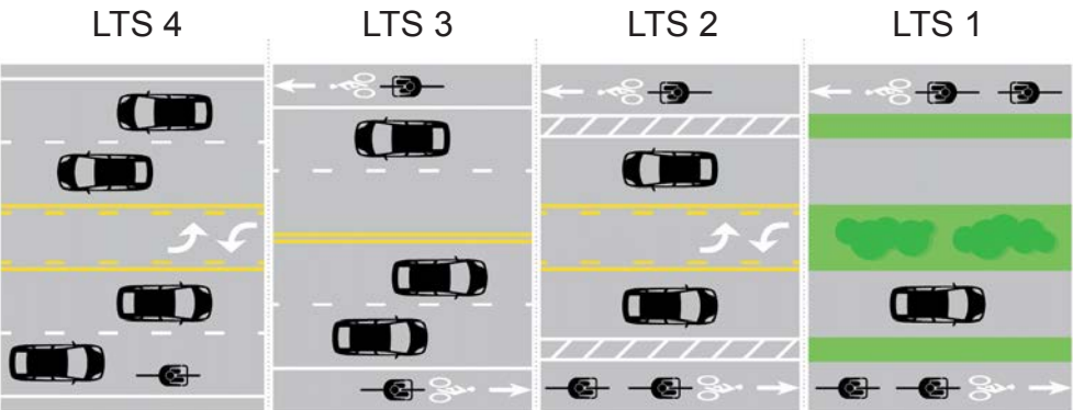
FIGURE 8. EXAMPLE ROADWAY CONFIGURATIONS BY LEVEL OF TRAFFIC STRESS
