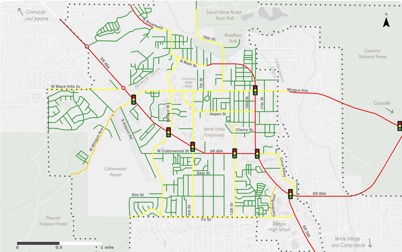
FIGURE 7. LEVEL OF TRAFFIC STRESS ANALYSIS, COTTONWOOD
