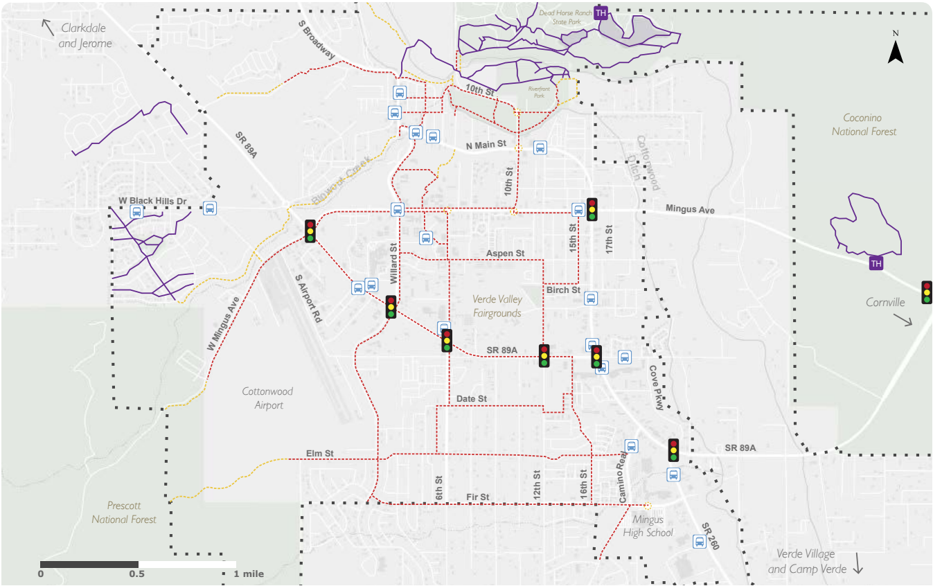
FIGURE 10. PROPOSED AND EXISTING TRAIL SYSTEM
